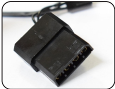
CONECTOR MOLEX
